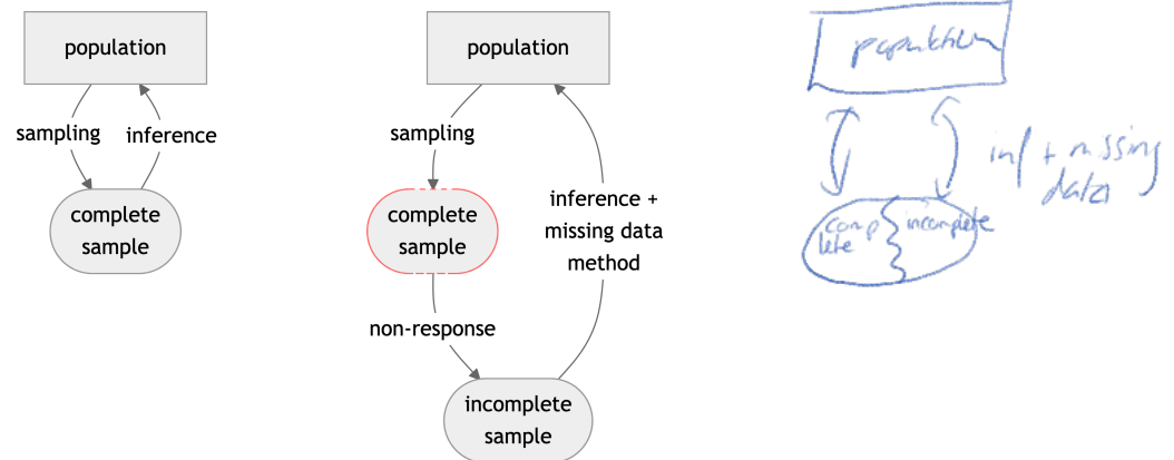
Figure 2: Inference with incomplete data
